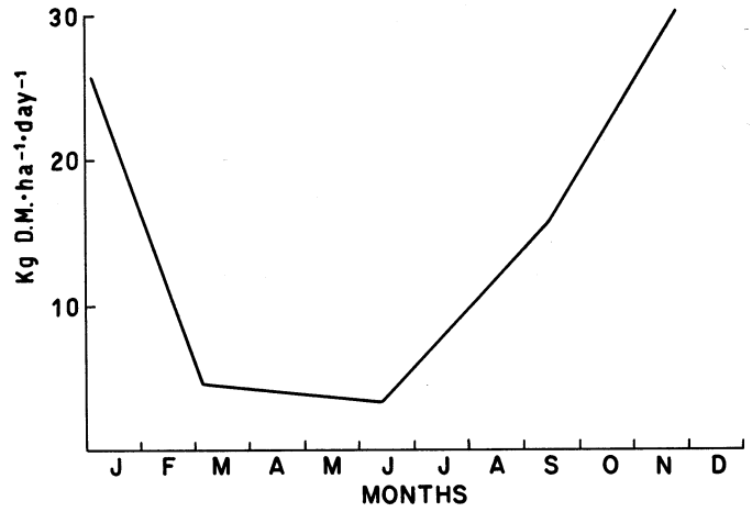
Fig. 6. Total aerial net primary productivity (ANPP) throughout the year.
