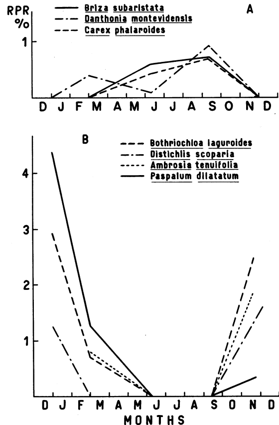
Fig. 7. Relative Productivity Rate (RPR) of the principal species. (a) cool-season (CS) species; (b) warm-season (WS) species.
