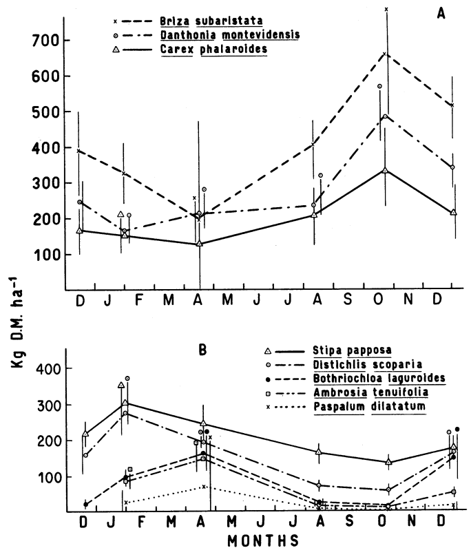
Fig. 2. Green biomass of the most important species during 1 year. Vertical lines represent 95% confidence intervals for means. (a) cool-season (CS) species; (b) warm-season (WS) species.
