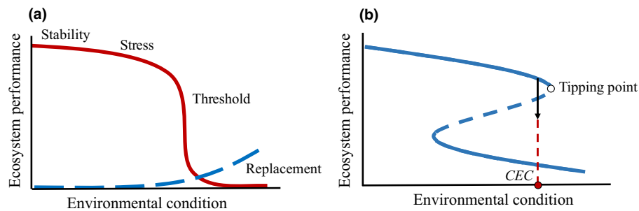
Fig. 1 There are multiple definitions of ecosystem thresholds, tipping points, and critical transitions. (a) A more general definition identifies a progression from ecosystem stability, to stress, to threshold response, and eventually to replacement by a novel ecosystem under changing environmental conditions. (b) A sensu strictu definition identifies alternative states of ecosystem performance, separated by an unstable equilibrium (dashed line) at a critical environmental condition (CEC; sensu Scheffer et al. , 2001). Returning environmental conditions to a previous level does not always result in the previous state of ecosystem performance. This figure was recreated from Scheffer et al. (2001) with permission from the Springer Nature Publishing Group.
